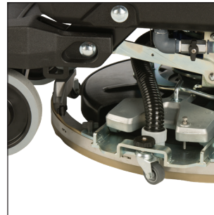
90° SQUEEGEE ROTATION in both directions, following the machine on every curve.
